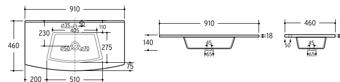
ROUND 90 910x460x140mm
