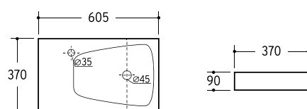
YOUNG 60 605x370x90mm
