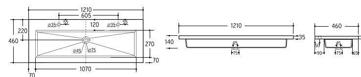
FASHION 120 1210x460x140mm
