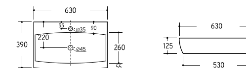
LAGO 63 630*390*125mm
