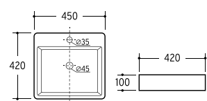
FLY 45 450x420x100mm
